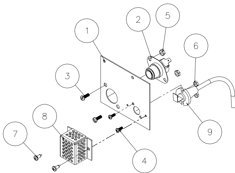
LOWERASSEMBLY
